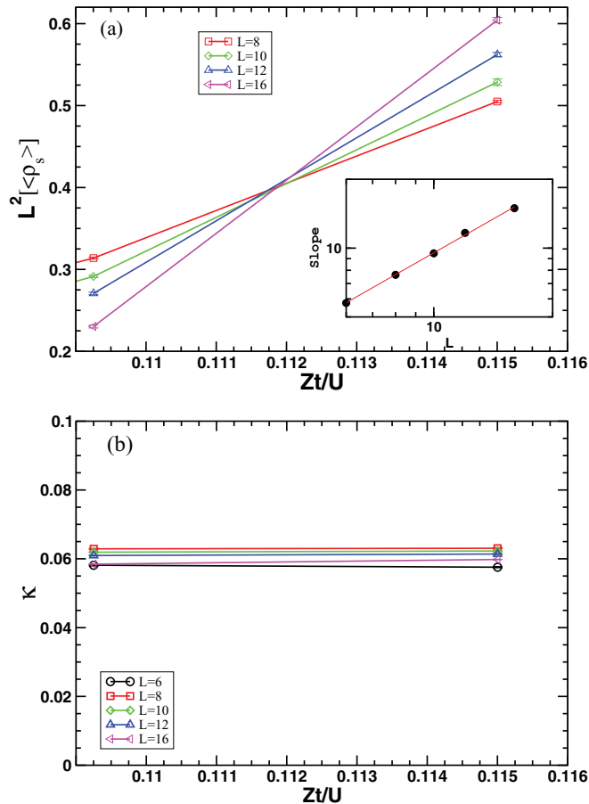
FIG. 8. (Color online) (a) Scaling curves of the superfluid density from grand canonical simulations at \mu/U = 0.375 . The inset shows the slope of these curves at the QCP on a log-log scale. (b) The compressibility \kappa in the same region.
