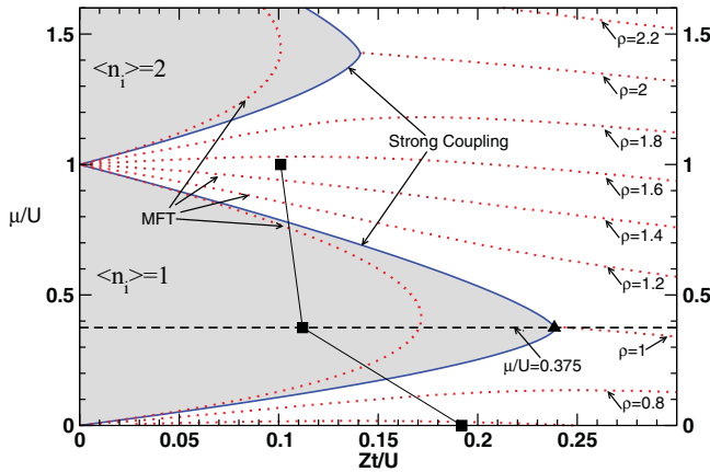
FIG. 1. (Color online) The phase diagram of the 2D Bose-Hubbard model. Shaded areas are the Mott insulating phases for zero disorder as determined from strong-coupling expansions in Refs. 37 and 38. The mean-field phase boundaries and constant density profiles for zero disorder are shown as red dotted lines. The dashed line indicates the constant chemical potential \mu/U = 0.375 . The solid triangle indicates the location of the transition to the Mott phase in the absence of disorder as determined by SSE simulations along the dashed line from Ref. 39. The three solid squares from bottom up are for the locations of superfluid to Bose-glass transitions in the presence of disorder at \mu/U = 0, 0.375, 1 , respectively, as determined from SSE simulations in this work.
