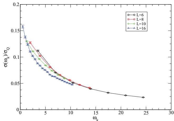
FIG. 7. (Color online) Dynamic conductivity scaling plot \sigma(\omega_k)/\sigma_Q vs Matsubara frequency \omega_k for Zt/U_c = 0.182 and t = 0.5 .
