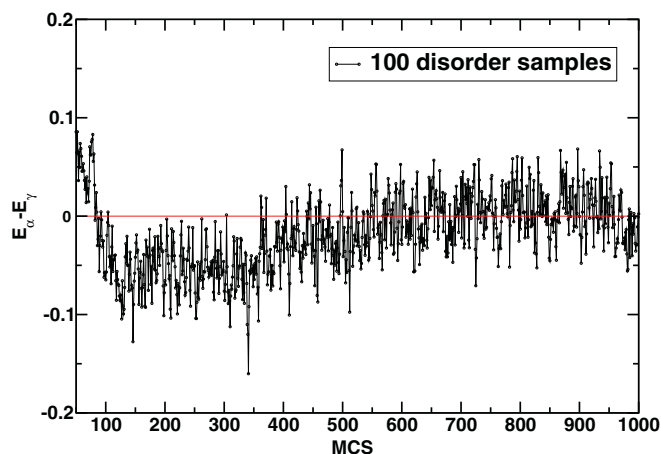
FIG. 3. (Color online) The energy difference between two replicas E_\alpha - E_\gamma as a function of MCS averaged over 100 disorder samples. Results are shown for L = 16 , t = 0.5 , U = 11 , and \beta = 12.8 . We start recording the energy difference after 50 MCS.
