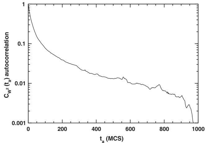
FIG. 4. The autocorrelation function C_{W^2}(t_a) for W^2 averaged over 100 disorder samples for L = 16 , t = 0.5 , U = 11 , and \beta = 12.8 . Note that the y axis is on a log scale.
