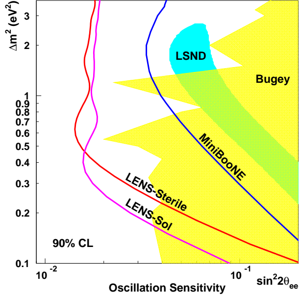
FIG. 3: Exclusion plots of sensitivity to active-sterile oscillations in LENS (with 4 \times 100 day exposure to 10 MCi Cr source) compared to those for LSND, BUGEY, and the projected sensitivity of MiniBooNE [16]. LSND and MiniBooNE are plotted assuming the best fit U_{e4} and U_{\mu 4} from Ref [4].
