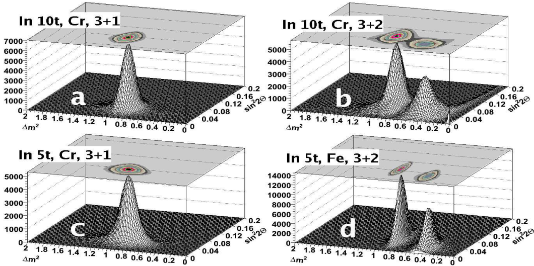
FIG. 2: Analysis of 3+1 and 3+2 models of sterile neutrinos in LENS. In 10t=8% In LENS-Sol ( A ); In 5t=15% In LENS-Sterile ( B ); Cr=4 MCi×100 days exposure to 51 Cr; and Fe=10 MCi×2 years exposure to 55 Fe.
