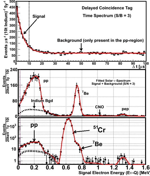
FIG. 1: Simulated 5 year-solar \nu_e signal spectra in LENS. Top panel: delayed coincidence time spectrum fitted to the isomeric lifetime \tau=4.76 \mu\text{s} . Middle panel: energy spectrum (with \sim 2000 pp events) at delays < 10 \mu\text{s} , and random coincidences (from the pure \beta -decay of In target) at long delays. Bottom panel: Spectrum from 4 \times 100 day exposure to a 10 MCi source of ^{51}\text{Cr} with the scaled solar spectrum included. The Cr signal has 1.3 \times 10^4 events with \sim 0.1\% background (from the ^7\text{Be} line).
