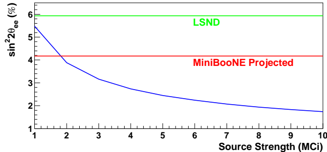
FIG. 4: Sensitivity to sterile oscillations vs ^{51}\text{Cr} source strength. The projected MiniBooNE sensitivity can be achieved with a source of less than 2 MCi.
