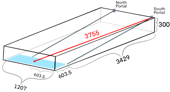
FIG. 4. South Portal detector to repository center. Measurements are in meters.
