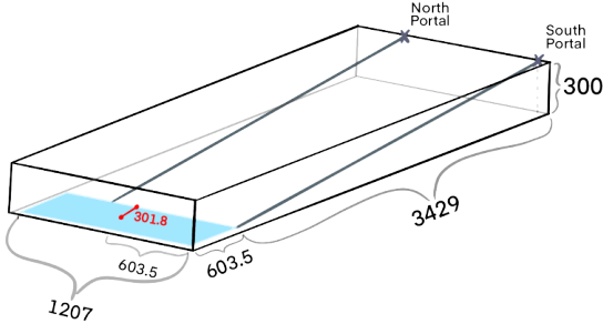
FIG. 5. Repository edge detector to repository center. Measurements are in meters.
