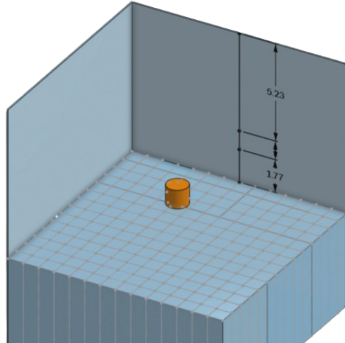
FIG. 3. Detector suspended above center of storage. Measurements are in meters.
