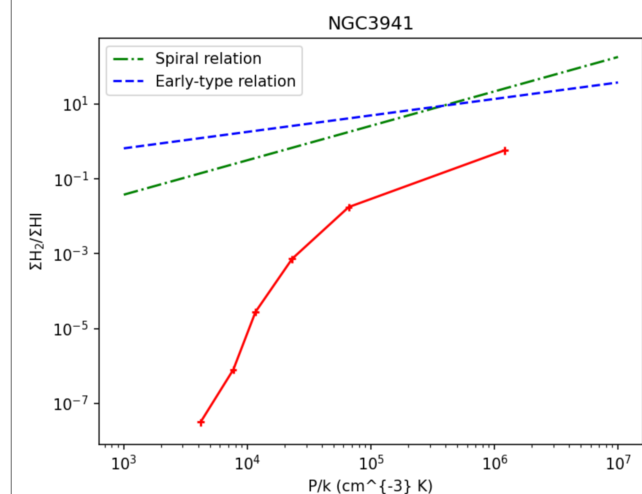
Figure 6: Depiction of the Midplane Pressure to H 2 /HI ratio. Blue represents the recent relation for early-type galaxies, Green is the relation for spiral galaxies (Walter et al., 2008).
