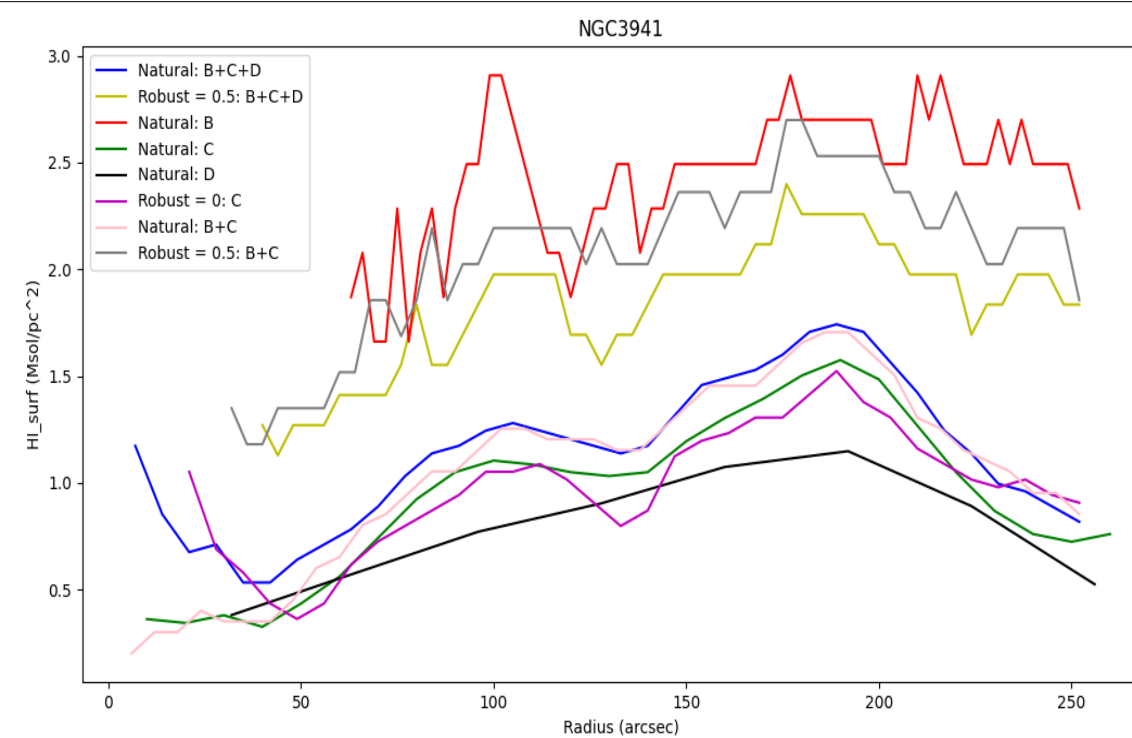
Figure 5: The radial HI surface density distribution derived from azimuthal averages in the HI maps. Key Features: A peak at 0 arcsec, a dip at 50 arcsec, and two other peaks at 100 and 175 arcsec indicate two rings of hydrogen within NGC 3941. Higher resolution images detect higher density HI, but resolve out the more diffuse HI in the center.
