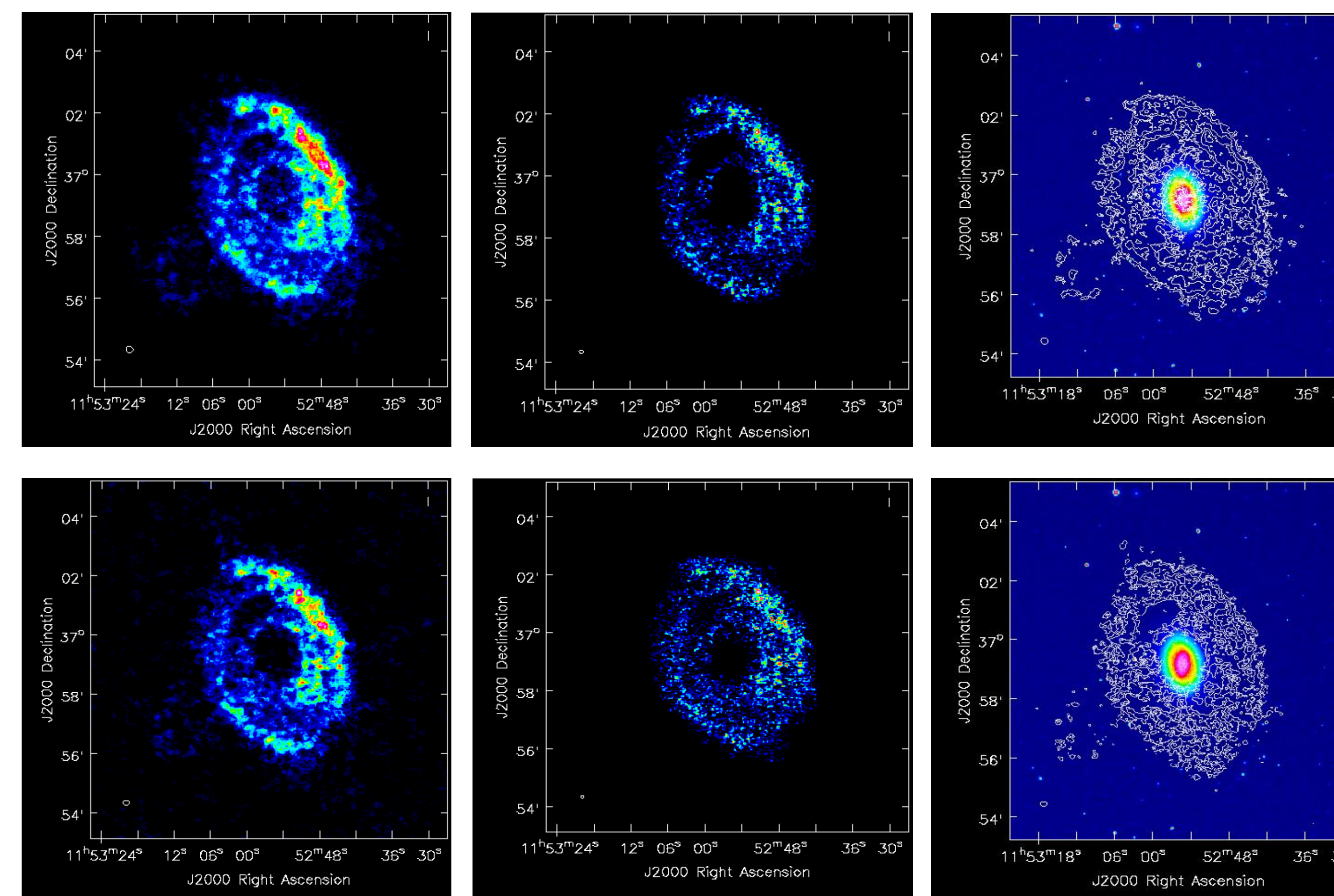
Figure 4: Moment/Contour maps of the HI content in NGC 3941 Top: B+C+D array Natural (14''), Robust (8''), Natural Contour Map Bottom: B+C array Natural (12''), Robust (7''), Natural Contour Map Key Features: Two HI rings are observed and an HI hole is at the center of the galaxy with some HI at the center. A companion dwarf galaxy is also seen.
