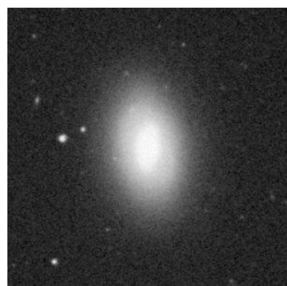
Figure 1: Digital Sky Survey image of NGC 3941 in R band. The galaxy is 12.4 kpc in diameter and is located in Ursa Major (McGlynn et al., 2008).
